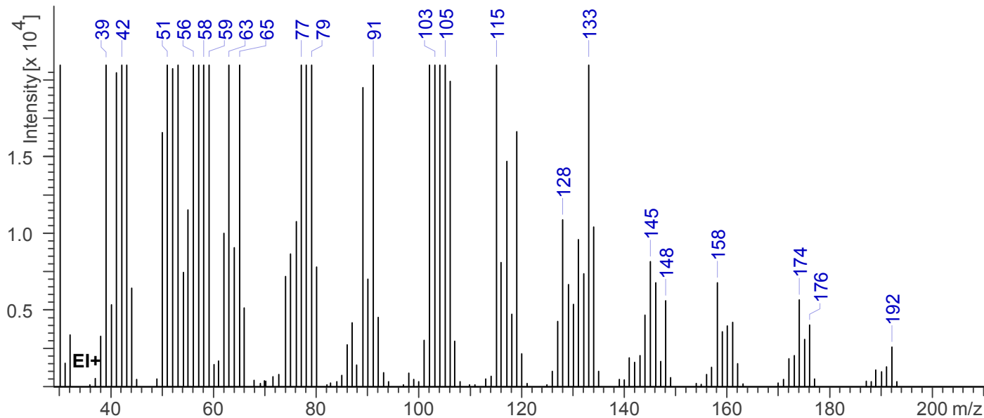
EI Mass Spectrum, 2,5-DMMC HCl Lot N17-P95D
