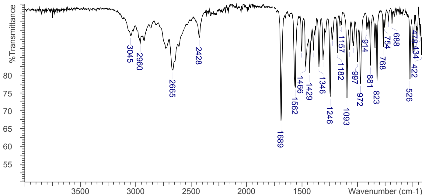
FTIR, ATR (Diamond, 3 Bounce) 2,5-DMMC HCl Lot N17-P95D
