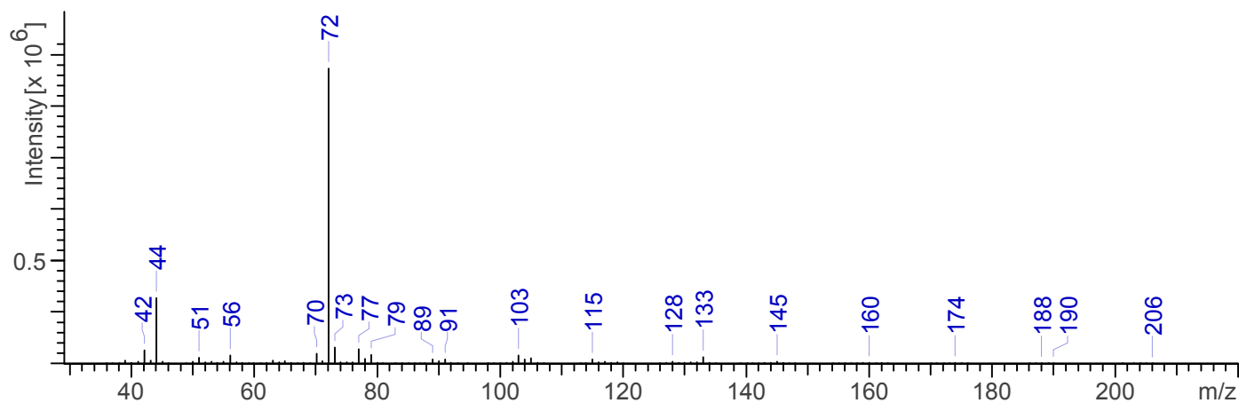
EI Mass Spectrum: 2-ethylethcathinone HCl; lot 0439301-1
