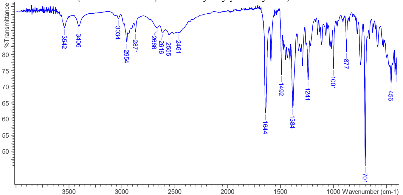
FTIR ATR (Diamond 1 Bounce): cis -3-methylbutyryl fentanyl HCl; Lot# 0535128-1
