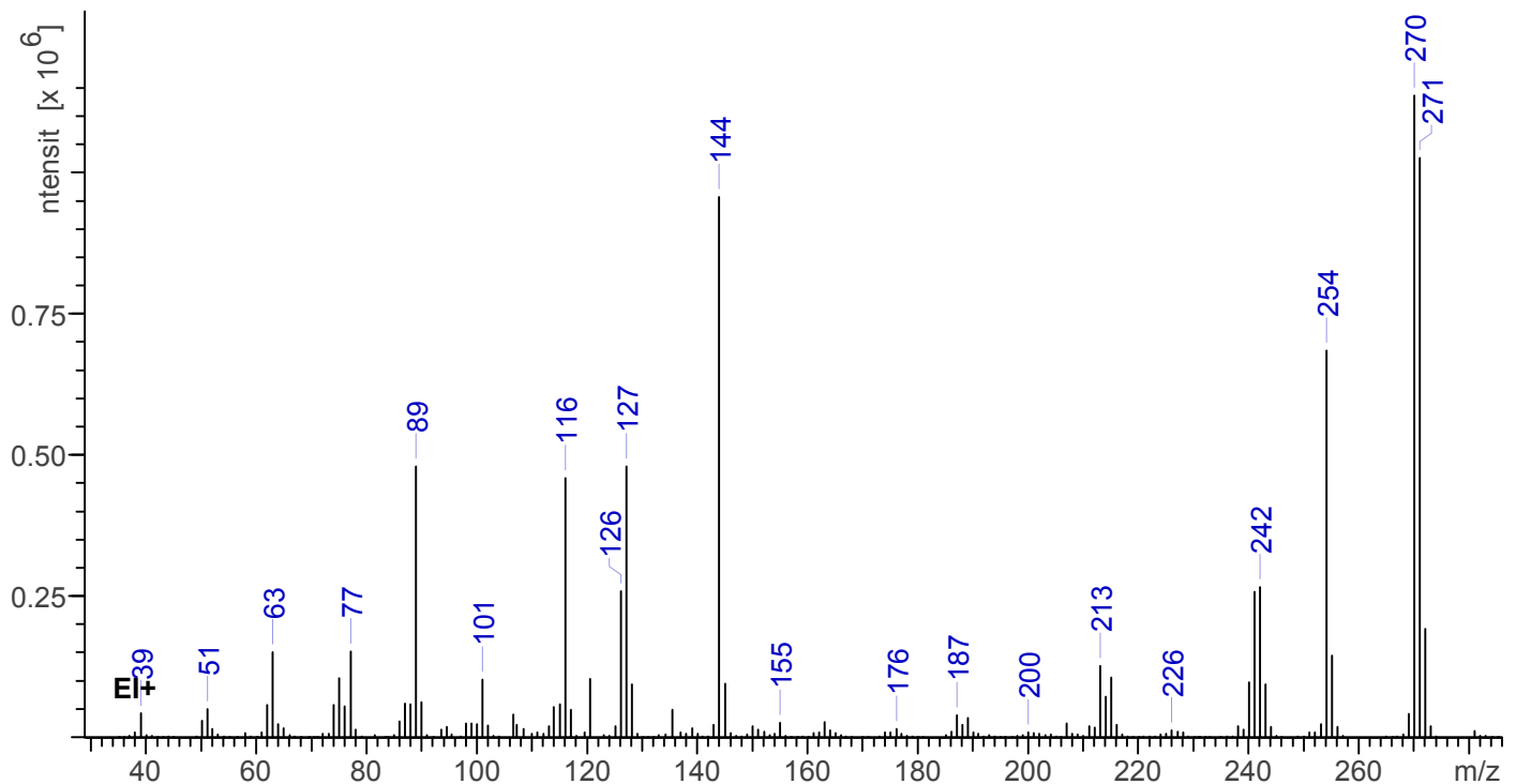
EI Mass Spectrum: 3-Naphthoylindole Lot# ALB213-15
