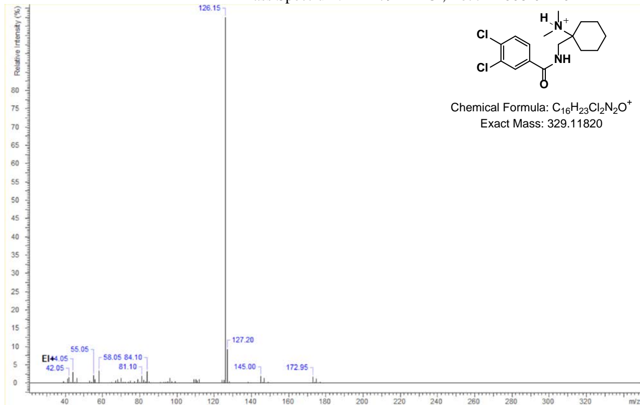
EI Mass Spectrum: AH-7921 HCl; Lot JLK008-041-01
