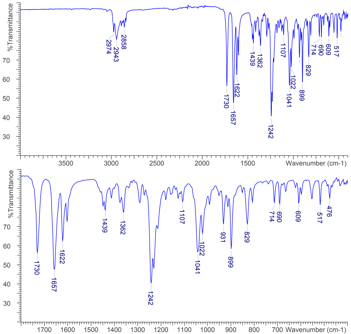
FTIR ATR (Diamond, 1 Bounce): Boldenone Acetate Lot#S267
