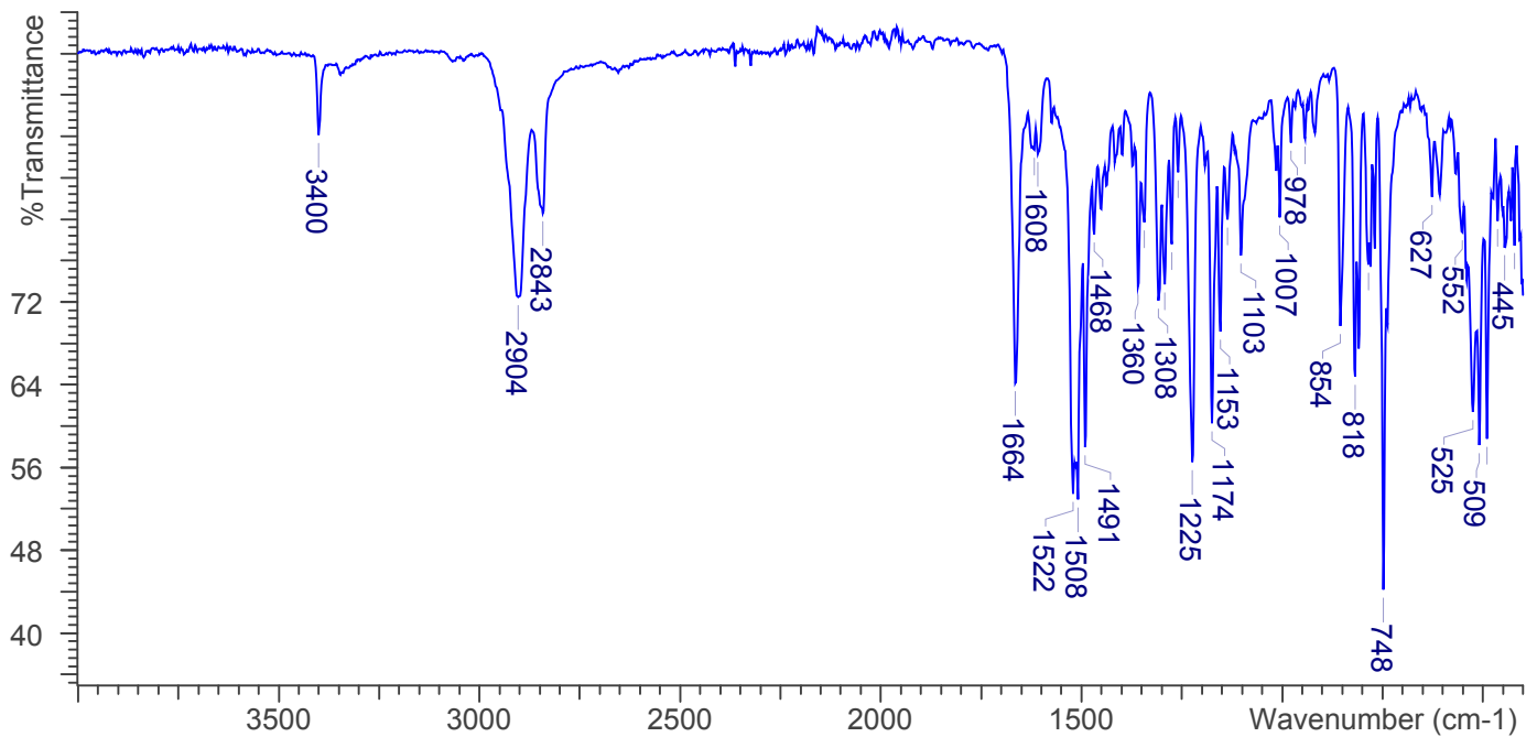
FTIR ATR (Diamond, 1 Bounce) FUB-AKB-48 Lot RM-131029-01
