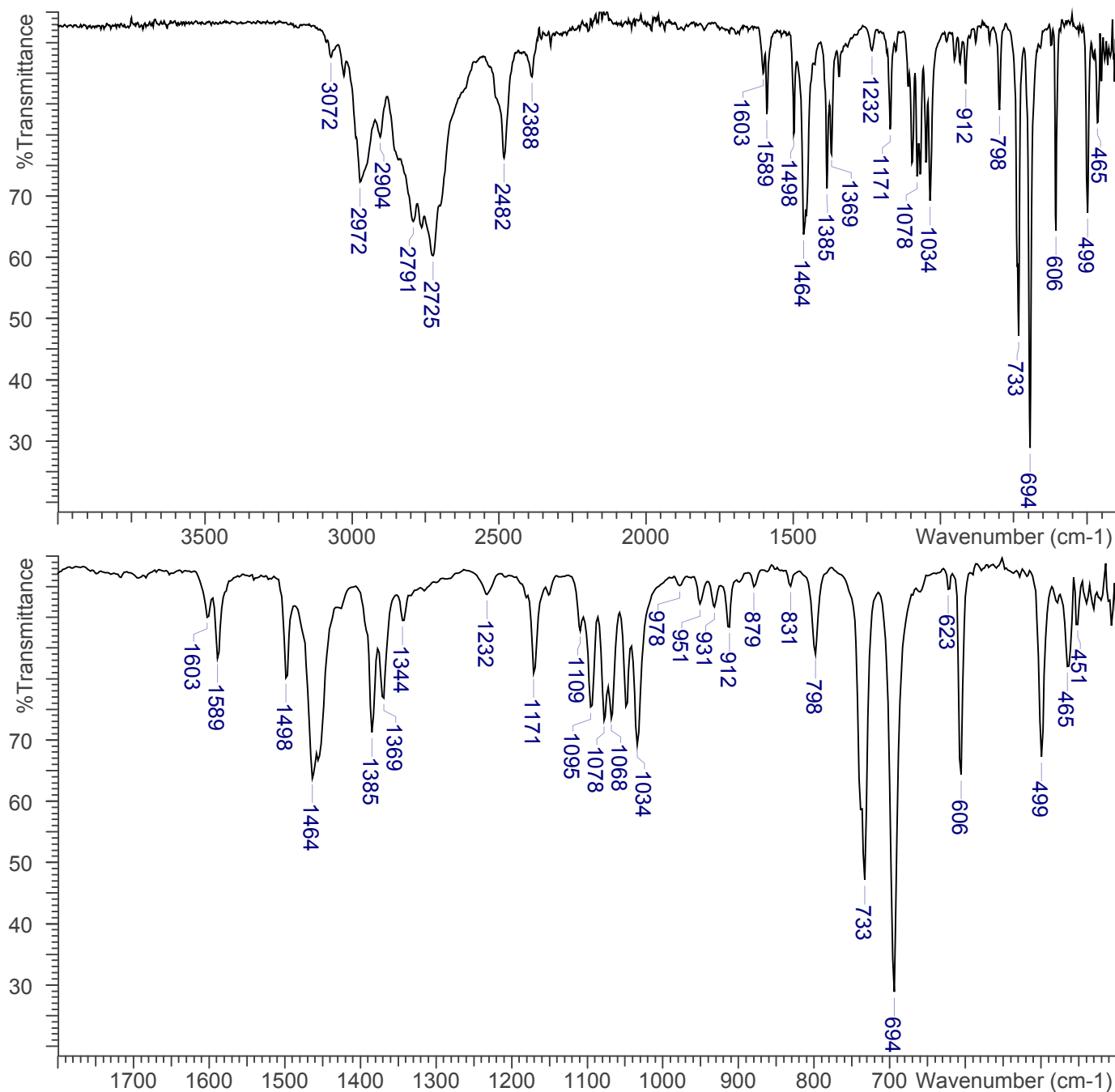
FTIR ATR (Diamond, 3 Bounce): N-ethylamphetamine HCl; Lot 2TDM-164-01
