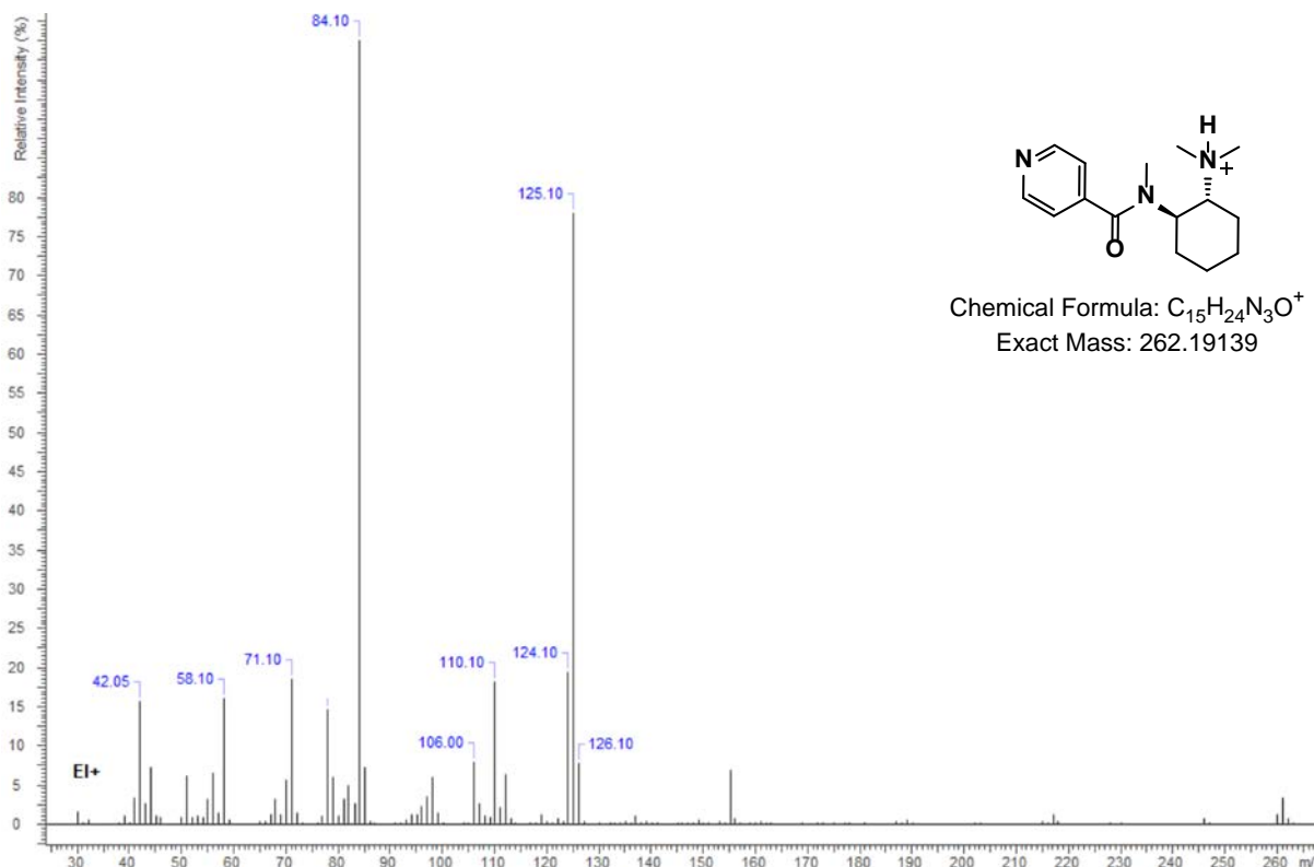
EI Mass Spectrum: U12 HCl; Lot JLK008-137-U12
