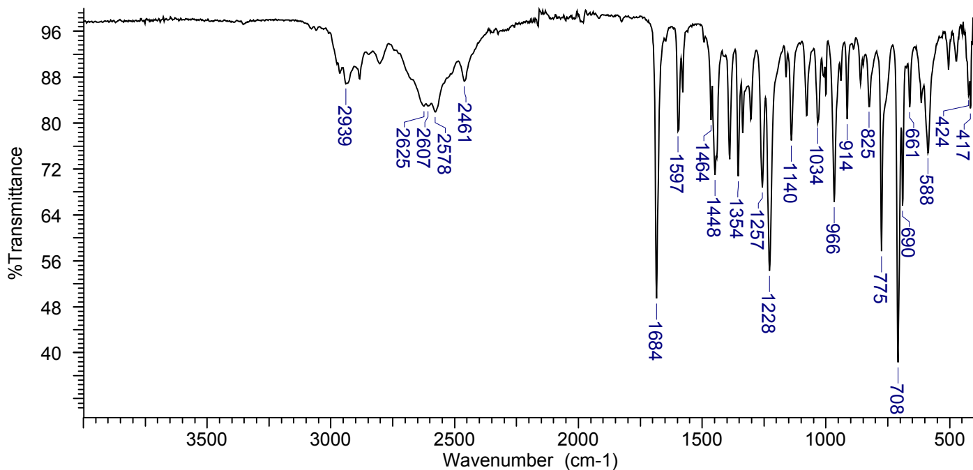
FTIR ATR (Diamond, 3 bounce): \alpha -PBP HCl; Lot ALB 225-2
