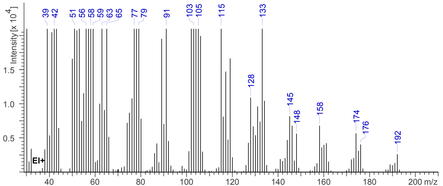
EI Mass Spectrum, 2,5-DMMC HCl Lot N17-P95D
