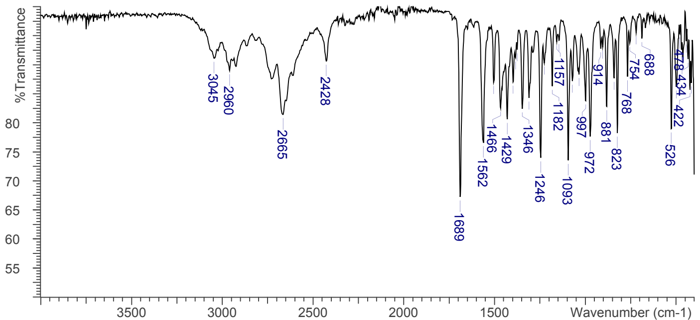
FTIR, ATR (Diamond, 3 Bounce) 2,5-DMMC HCl Lot N17-P95D
