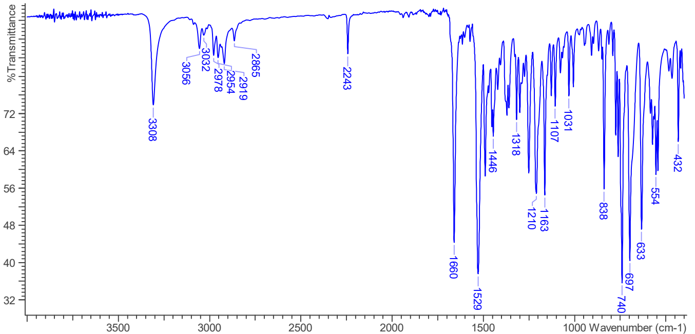
FTIR ATR (Diamond 1 Bounce): 4-cyano CUMYL-BUTINACA; Lot# 0533353-2
