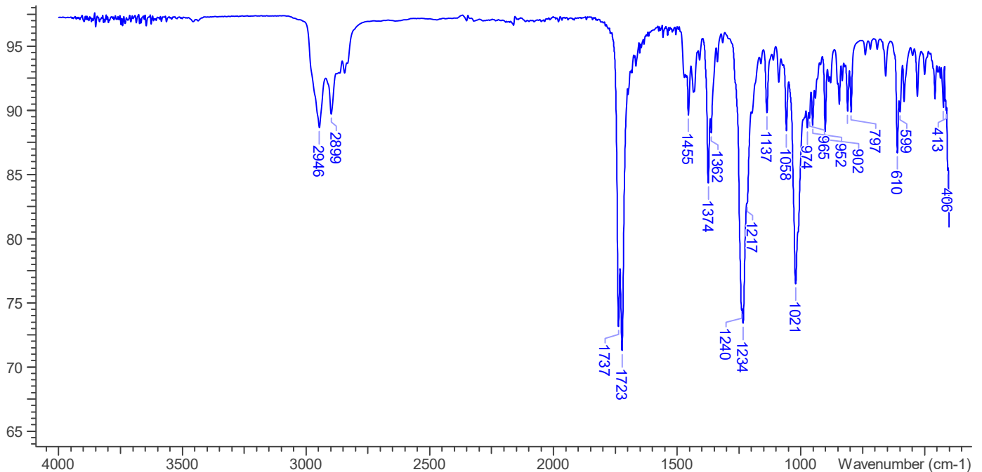
FTIR ATR (Diamond 1 Bounce): Dehydroisoandrosterone 3-Acetate; Lot#17984
